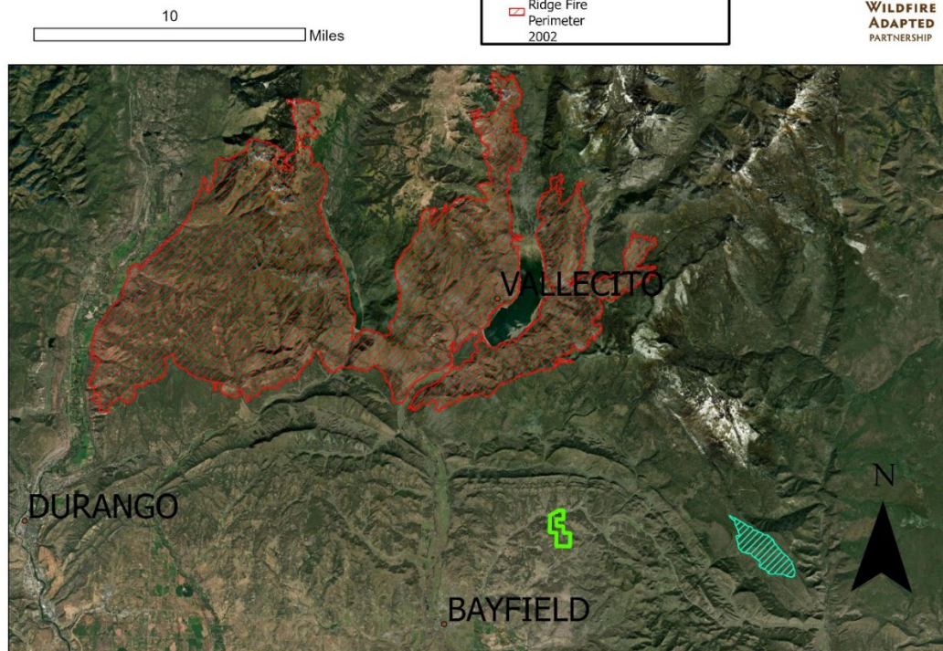
Figure 5: Missionary Ridge Fire and Dry Lake Fire Perimeter to DVE vicinity
